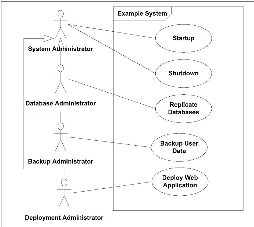
Figure 7-11. Actor generalization, in which the System Administrator is the generic base actor and the lower three are specializations
